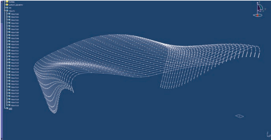
Fig. 2.8 A model developed with a parametric component called “Power Copy” in Digital Project, as it semi-automatically generates arc variations for the Gallery (Image by author)
